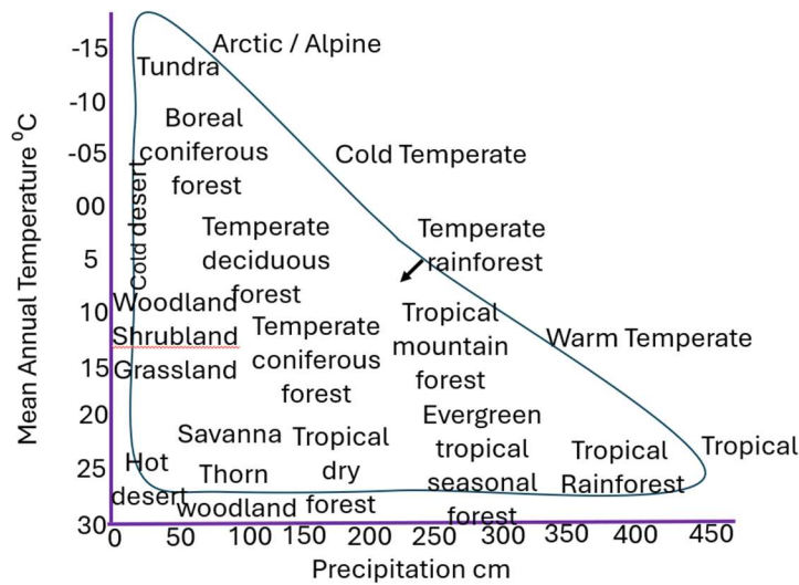
Figure 2. The distribution of global natural ecosystems in relation to mean annual temperature and precipitation. (modified by Alan Journet from Whittaker 1975)
