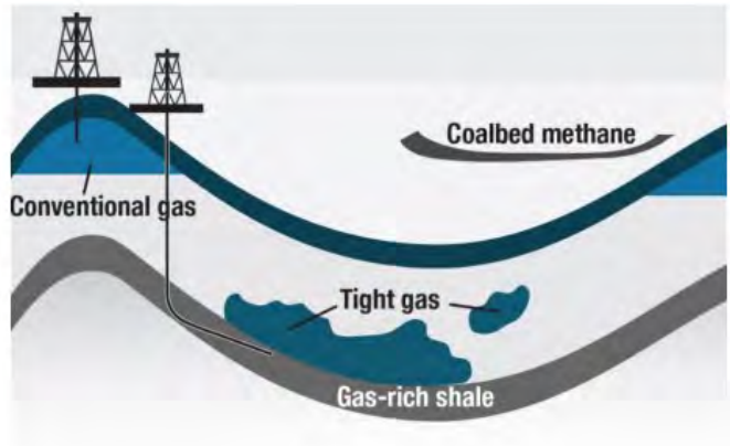
Figure 36: Where Natural Gas is Found 46
