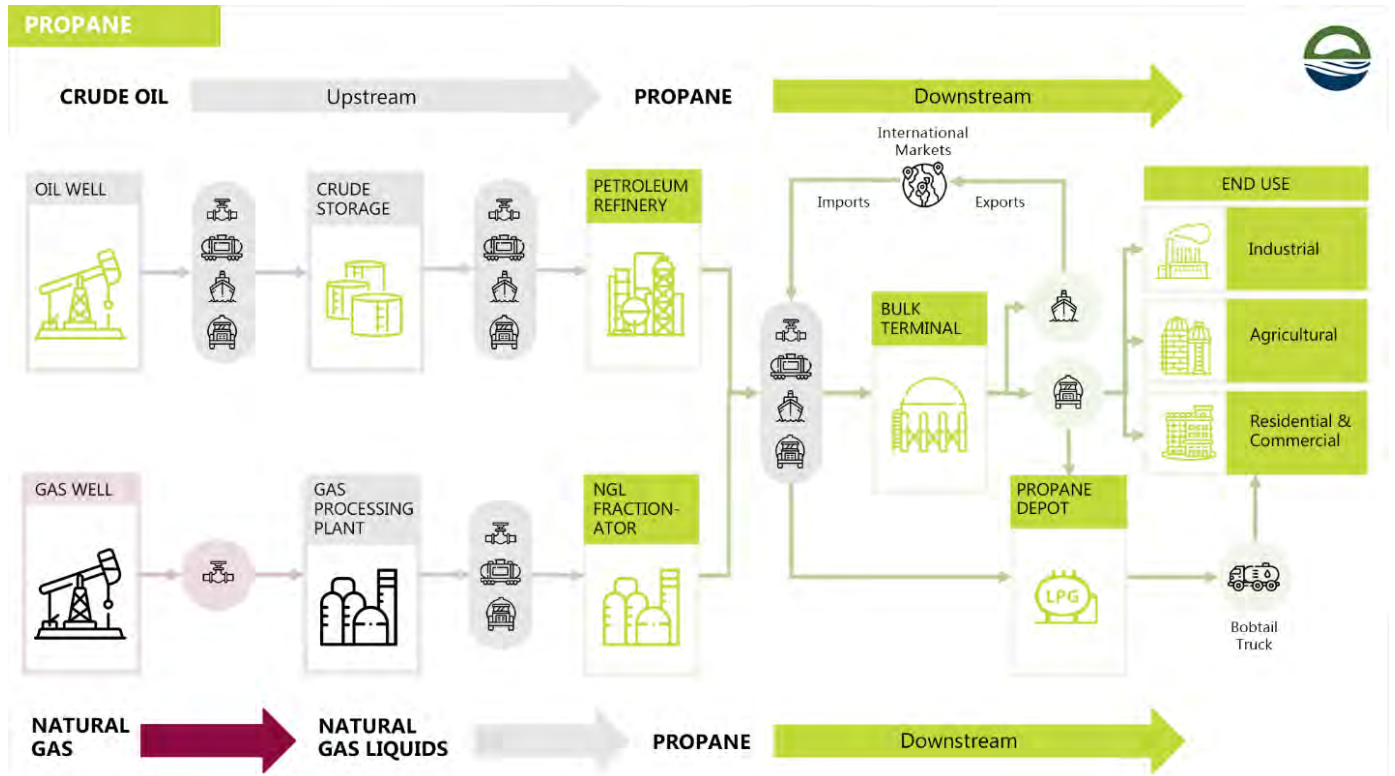
Figure 47: Propane Supply Chain
