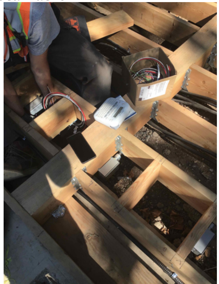
Lighting Rough-in
