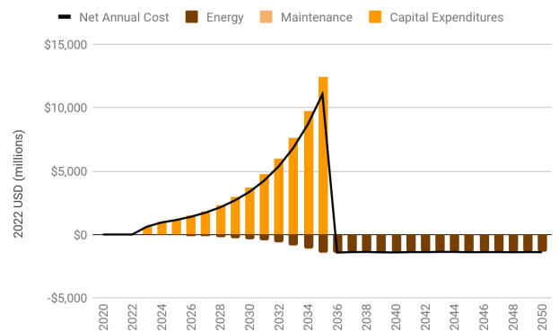
Figure 5: Energy Efficiency Policy scenario 2d, net annual costs or savings
