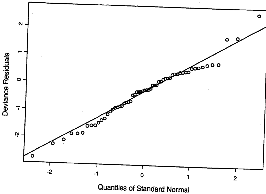
Fig. 20. Normal probability plot of deviance residuals from model in Fig. 19C.
