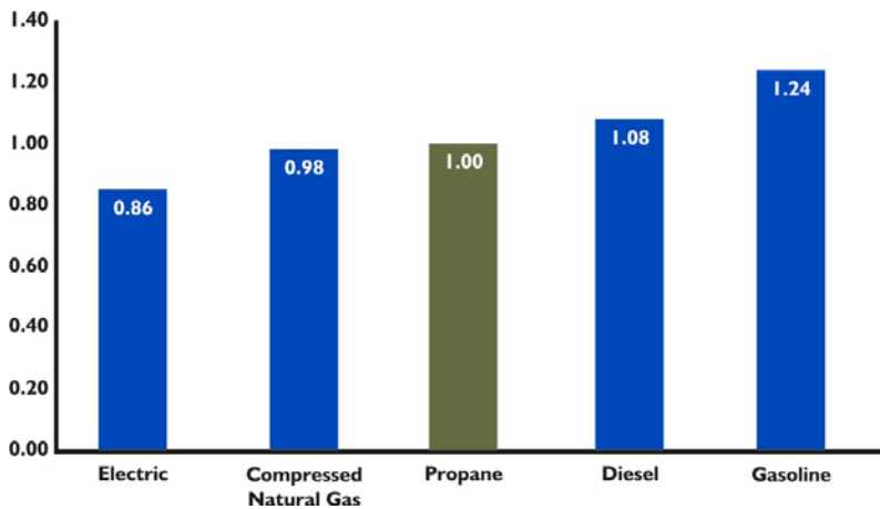
Figure 4.10. Forklifts
