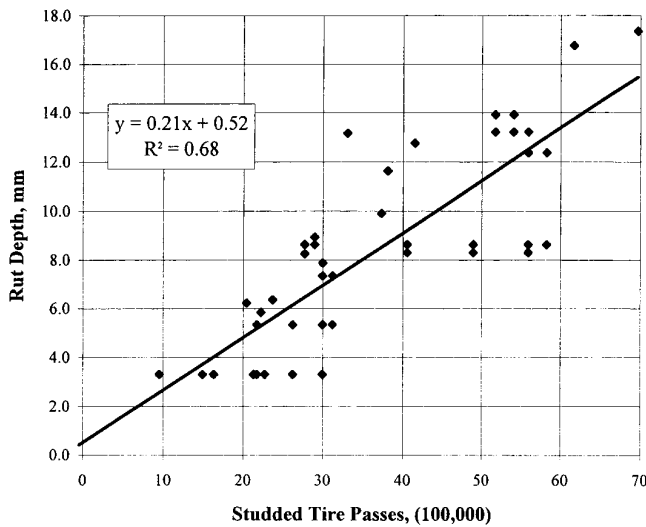
FIGURE 4 PCC studded tire wear rate results.
