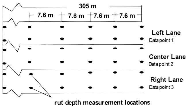
FIGURE 2 Rut depth measurement technique.
