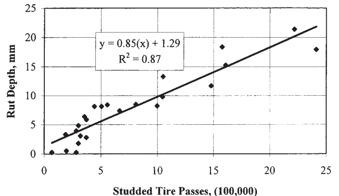
FIGURE 3 Asphalt studded tire wear rate results.
